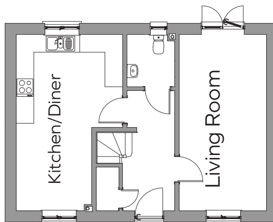
Plot 85 GROUND FLOOR PLAN
